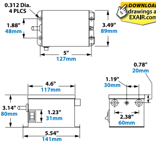
The Model 7901 and 7907 Power Supply has a lighted power switch and (2) 5kV outlets.
