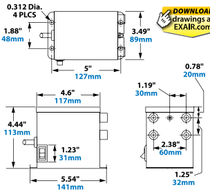
The Model 7940 and 7941 Power Supply has a lighted power switch and (4) 5kV outlets.
