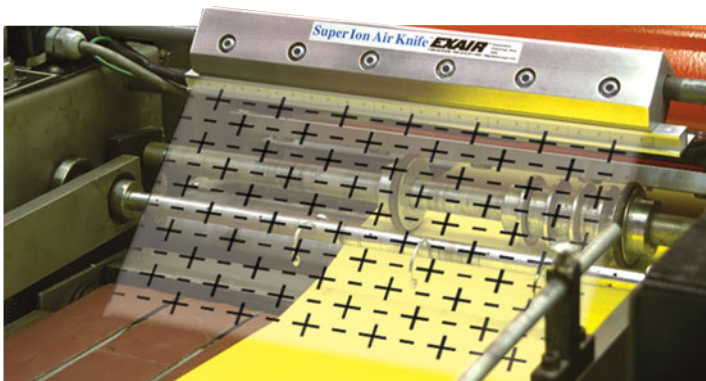
The Super Ion Air Knife eliminates static on a sheeter, so it picks up one sheet at a time.
